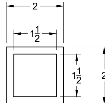
Front Scale = 1:2
