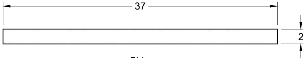
Side Scale = 1:8
